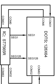
LCD LAYOUT
